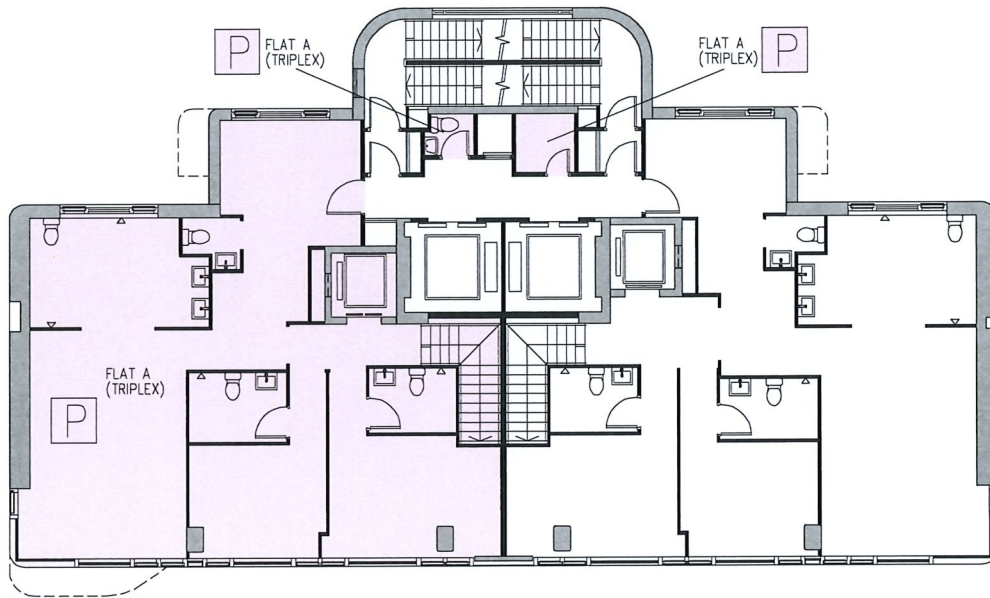
B/F, G/F, 1/F & 2/F FLAT A (TRIPLEX)
