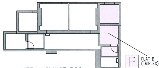
LIFT MACHINE ROOM PART PLAN
